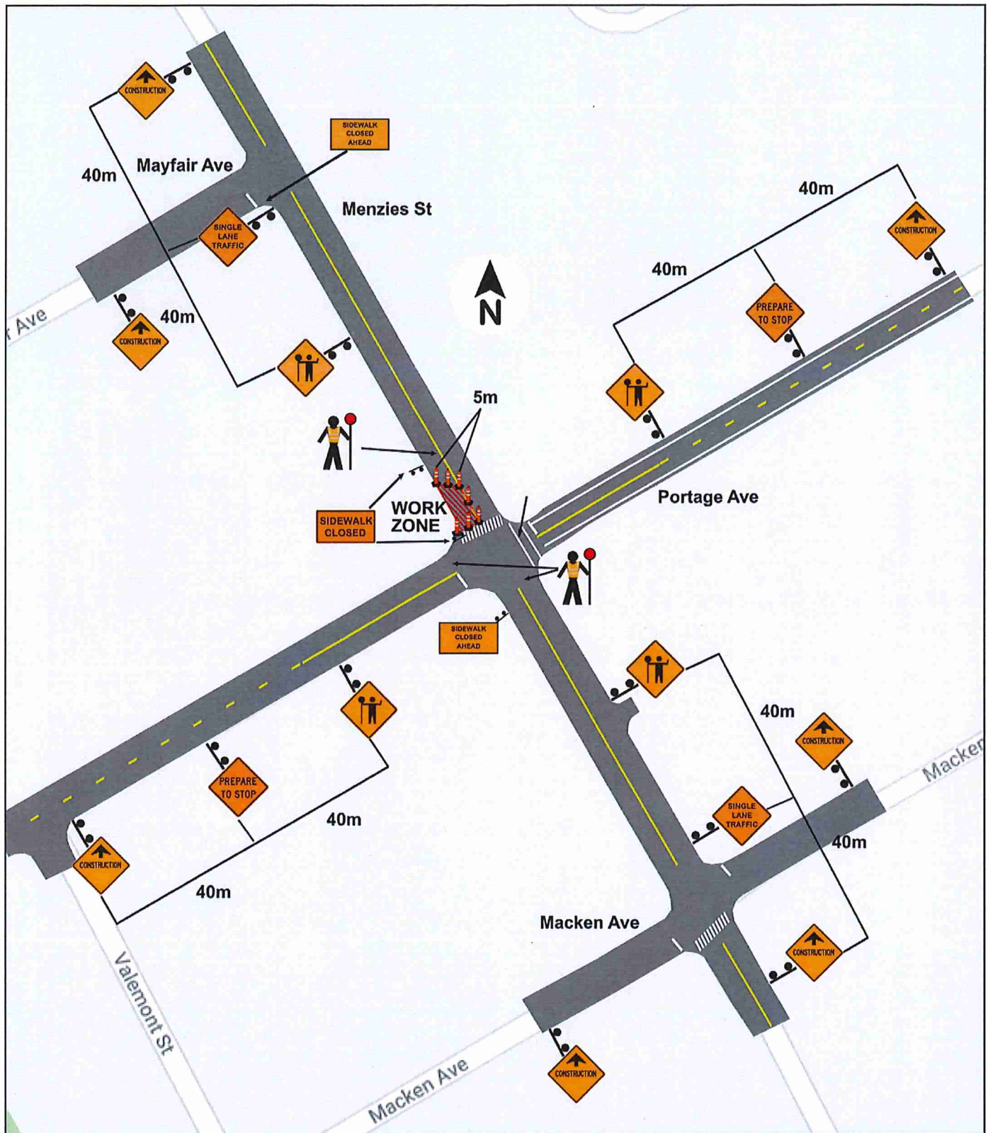
Figure 11.2: Intersection Lane Closure - Two-Lane, Two-Way Roadway with TCPs (Near Side) Short and Long Duration Letdown to stay clear for use during construction. TCPs on site to assist with vehicles, pedestrians, bicyclists and all others.
