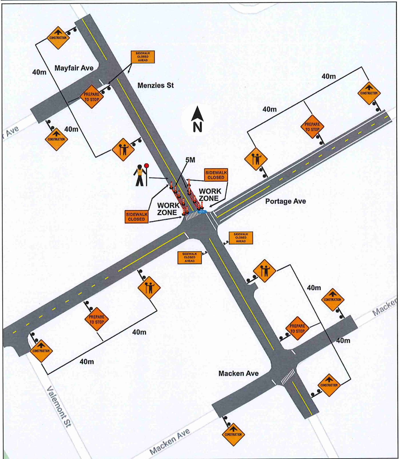
Figure 7.5: Work on Shoulder - Short and Long Duration Both closures shown - Only one side to be worked on at a time Letdown to stay clear for use during construction. TCP on site to assist with vehicles, pedestrians, bicyclists and all others
