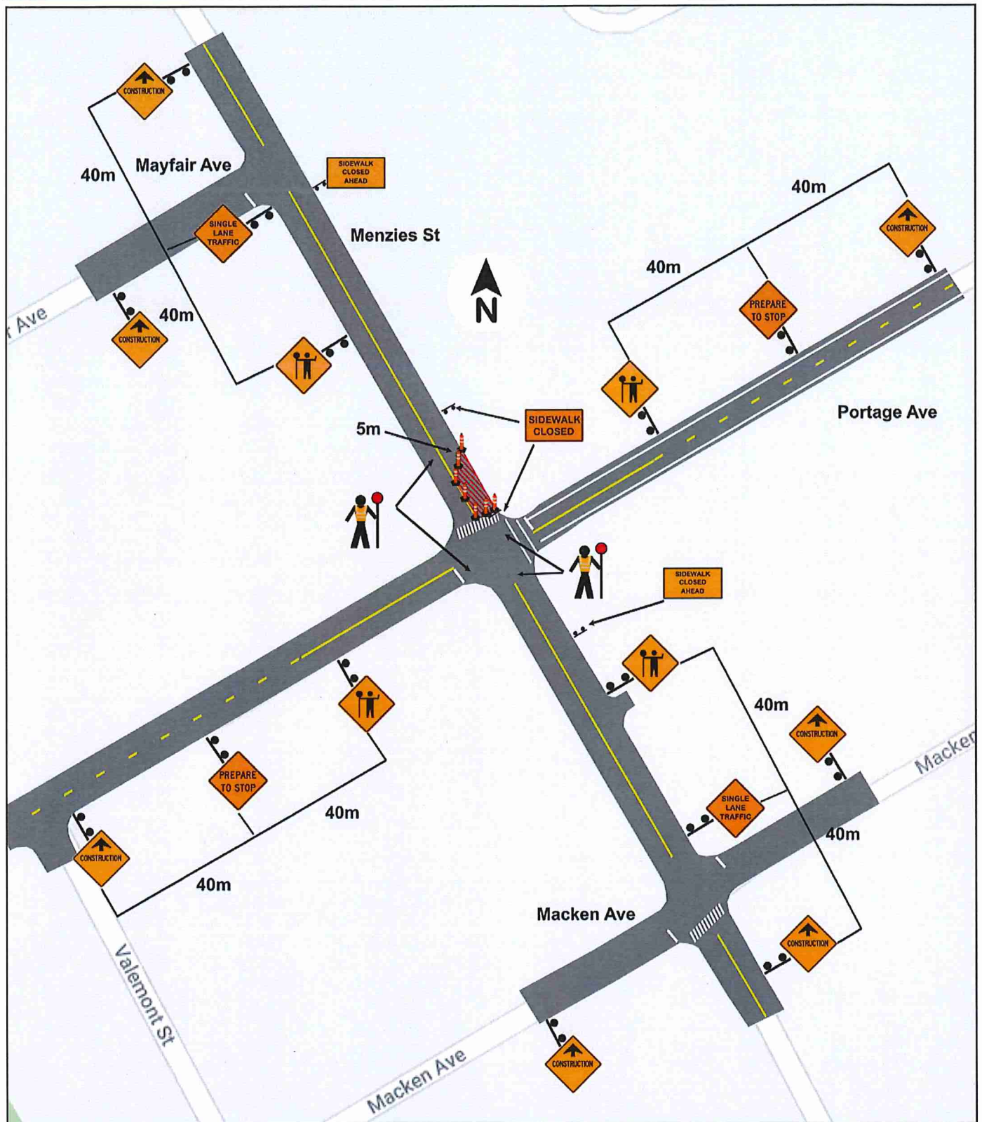
Figure 11.4: Intersection Lane Closure - Two-Lane, Two-Way Roadway with TCPs (Far Side) During letdown construction a temporary ramp will be built out of hard packed mulch on either side of the construction zone. During all other construction, the letdown will remain clear for use. TCPs on site to assist with vehicles, pedestrians, bicyclists and all others.
